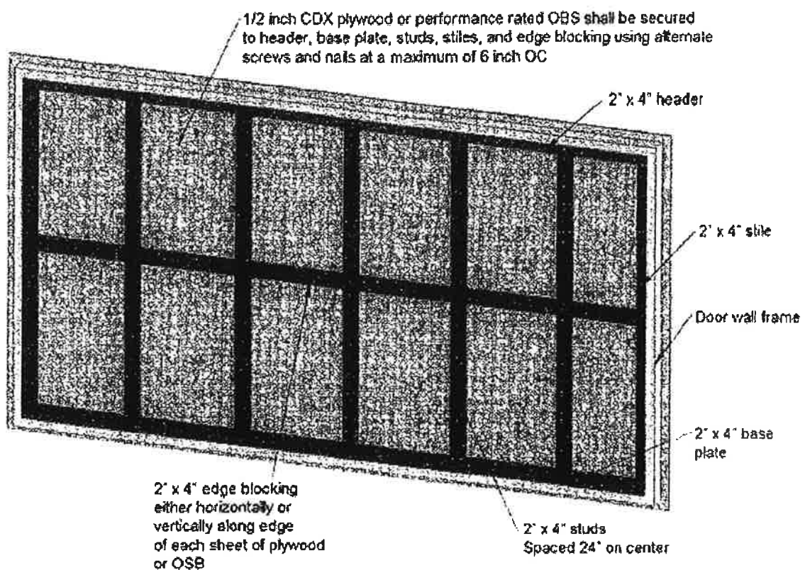
FIGURE A103.1(2) BOARDING OF DOOR WALL
